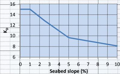
Graph 2-Relationship between the K_D stability coefficient and the seabed slope.
